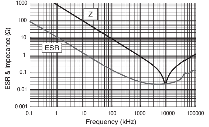
●KVF Series 100V/0.22 \mu F
