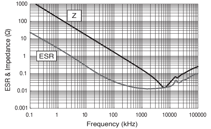
●KVF Series 100V/0.22 \mu F
