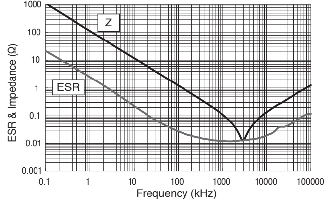
●KVF Series 50V/1.0 \mu F
