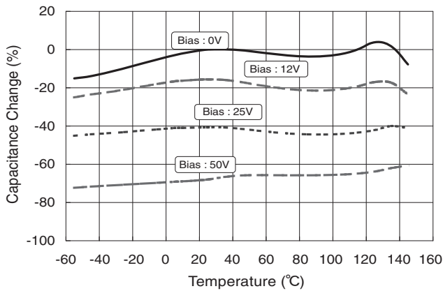
● NTS series (X7R) 100V
