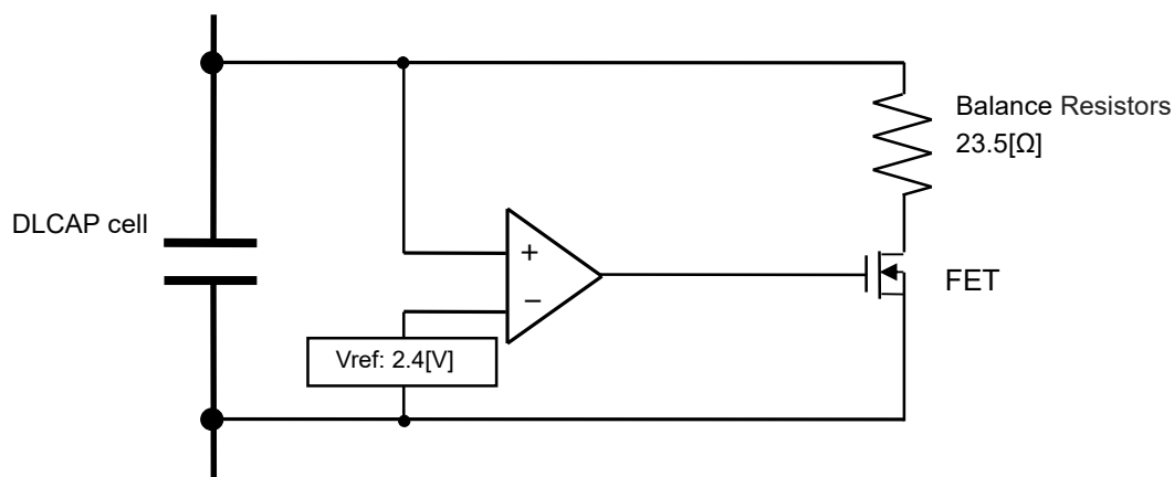
Figure 3-1. Schematic diagram of the balance circuit
