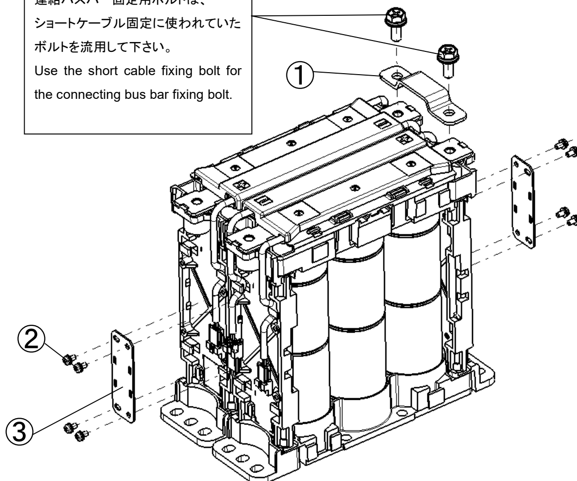
Figure 4-3. Outline of the module
