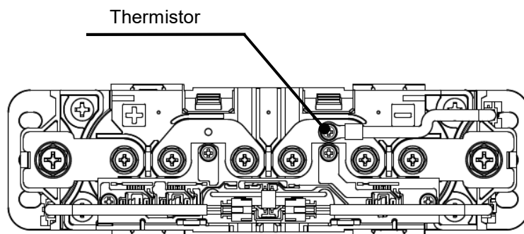
Figure 3-5. Thermistor position
