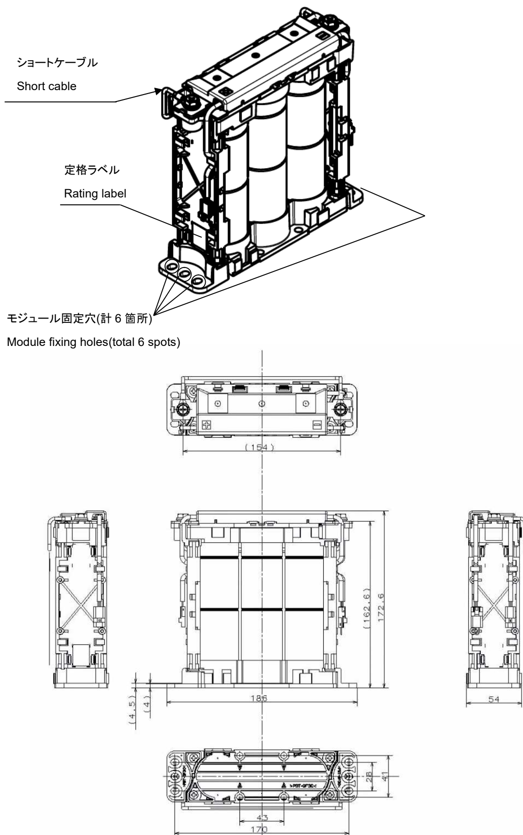
Figure 4-1. Outline of the module
