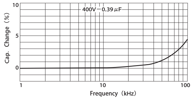
Capacitance-Frequency (at20°C)
