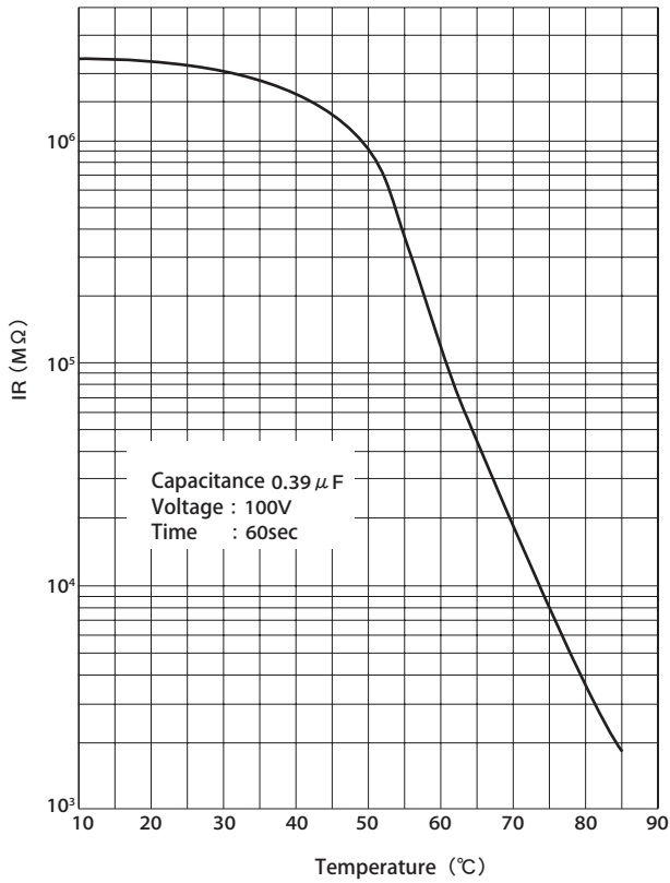
Insulation resistance-Temperature
