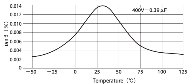
1 kHz Dissipation Factor (tan δ) -Temperature
