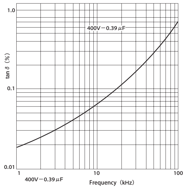
Dissipation Factor (tan δ) -Frequency (at20°C)
